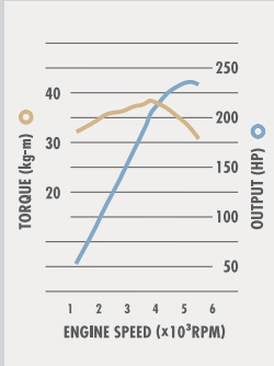
1GR-FE 4.0-litre Gasoline 235HP/5200rpm 38.3kg-m/3800rpm (Automatic Transmission)
